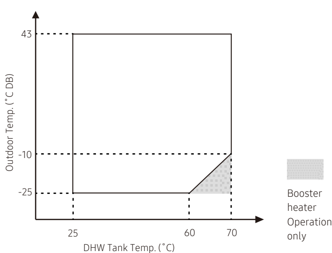
3) DHW (Domestic Hot Water Tank)
